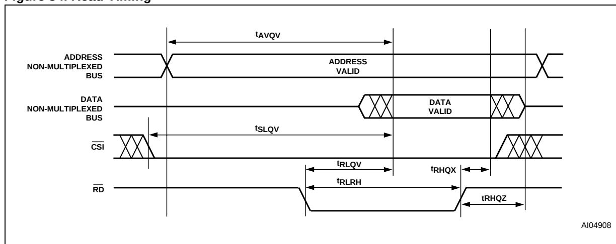
Figure 34. Read Timing
